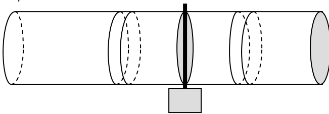
Round damper in-line with round duct.
