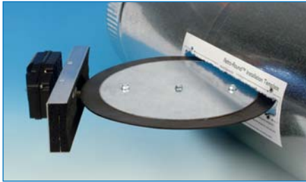
NEW Retro-Round™ Insertable Damper with Plug-In Motor Connections
